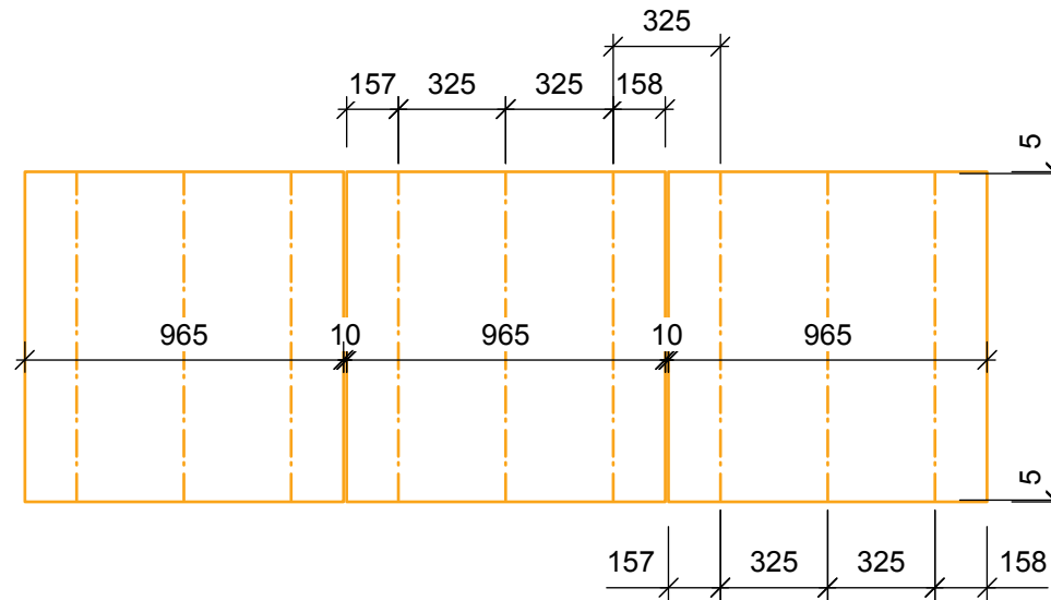
PATTERN "F"
